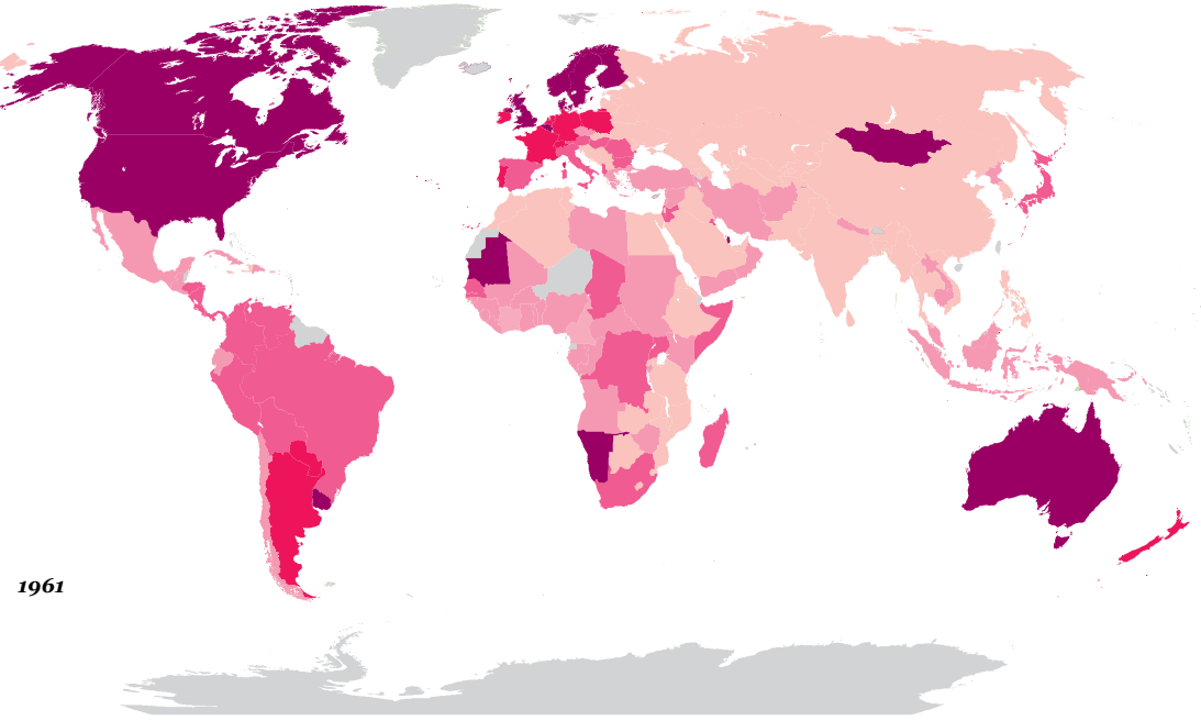
Figure 25: Changing Ecological Footprint per person Global map of national Ecological Footprint per person in (a) 1961 and (b) 2008 (Global Footprint Network, 2011).
