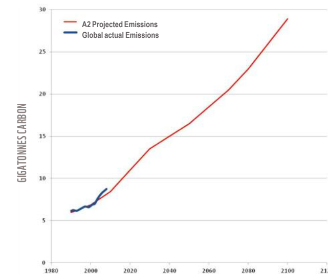
FIGURE 4.5 CARBON EMISSIONS PROJECTED BY THE INTERGOVERNMENTAL PANEL ON CLIMATE CHANGE (IPCC) SRES A2 SCENARIO (SEE SIDEBAR, GLOBAL CLIMATE MODELLING) AND ACTUAL GLOBAL CARBON EMISSIONS. Source: WWF, using data from IPCC 2000 and CDIAC 2011.
