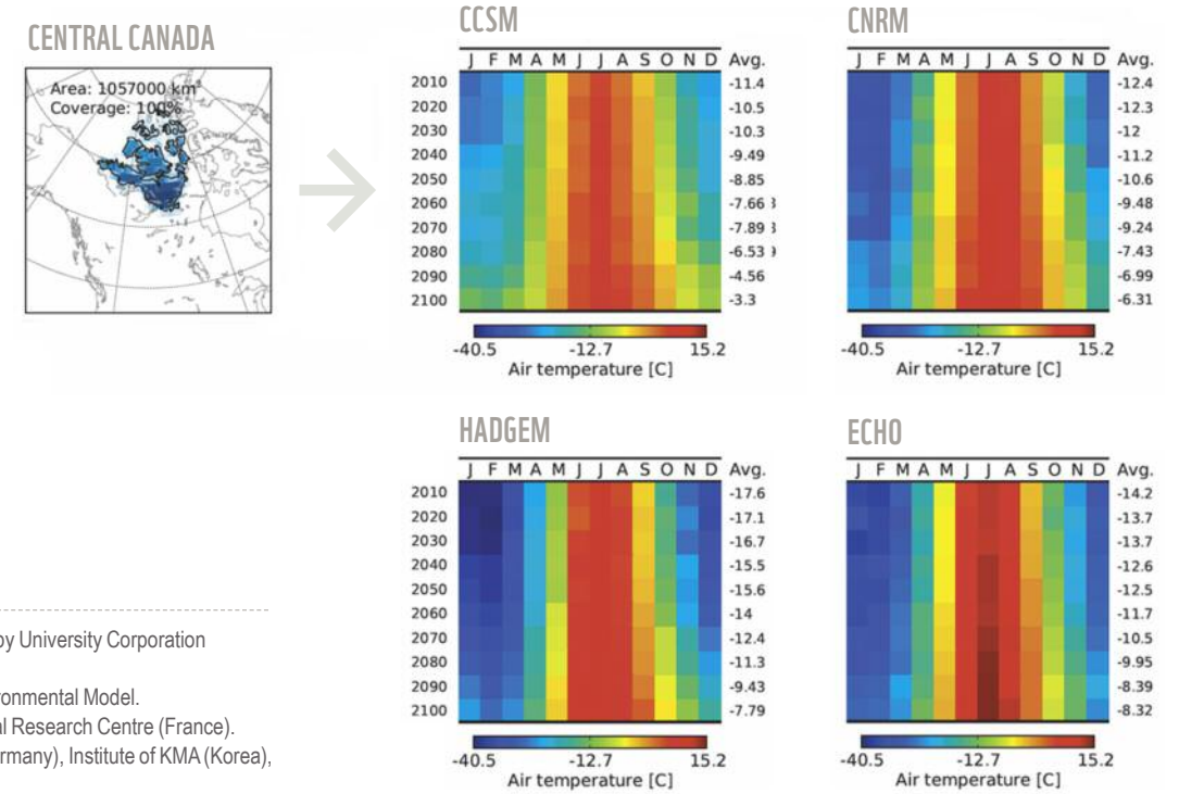
FIGURE 4.3 SURFACE AIR TEMPERATURE PROJECTED BY FOUR GENERAL CIRCULATIONS MODELS (GCMs) FOR THE CENTRAL CANADA ARCTIC ECOREGION. Source: Huard 2010.
